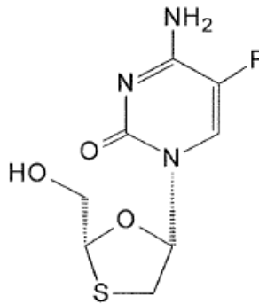
EMTRICITABINE
